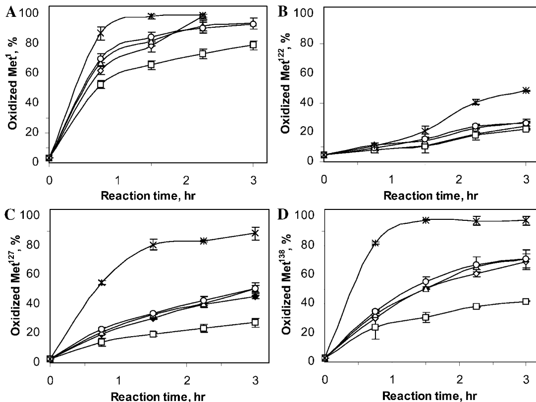
Fig. 2. Effects of different antioxidants on the oxidation of methionine residues in G-CSF: (A) Met 1 , (B) Met 122 , (C) Met 127 , and (D) Met 138 . (◇) control; (□) methionine; (△) glutathione; (○) acetylcysteine; (*) ascorbic acid. Oxidation reactions were carried out with 0.3 mg/ml G-CSF, 60 mM H 2 O 2 , 25 mM acetate, at pH 4.5 and 25°C. The concentrations of antioxidants are 60 mM.
